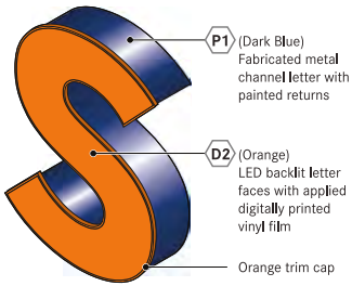
Isometric Channel Letter Detail
