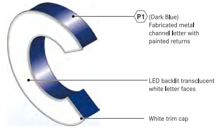
Isometric Channel Letter Detail
