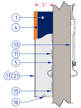
REMOTE "SUITES" LED CHANNEL LETTER PROFILE NOT TO SCALE
