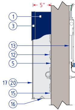
REMOTE LED LOGO PROFILE NOT TO SCALE
