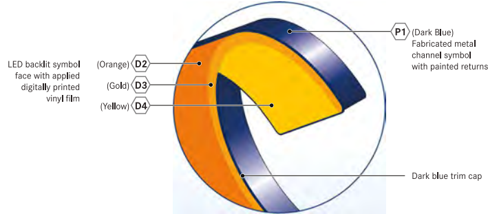
Isometric Symbol Detail
