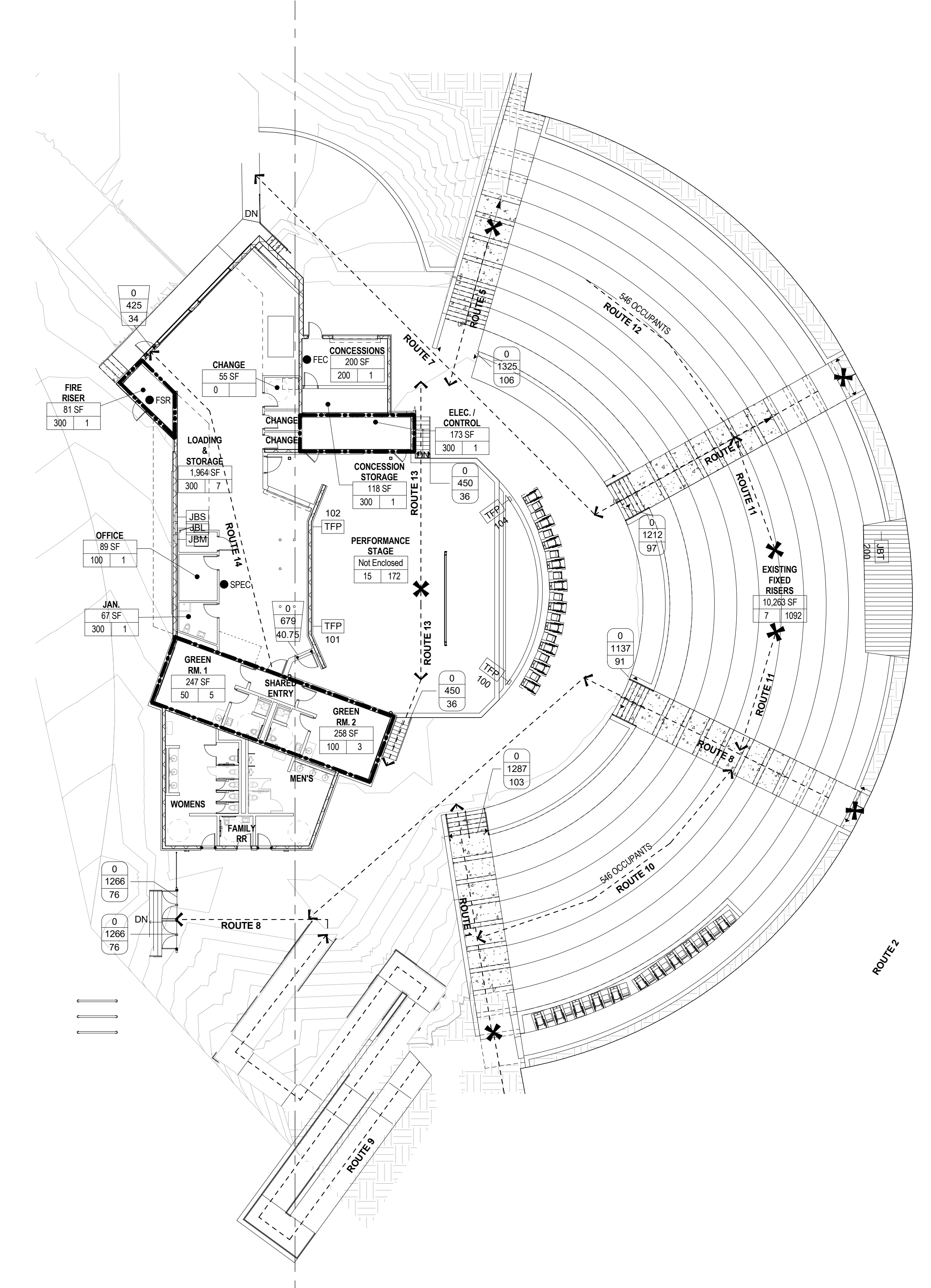
1 STAGE LEVEL LIFE SAFETY PLAN 1/16" = 1'-0"
